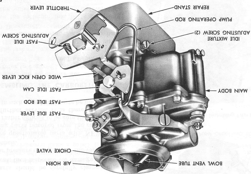
Fig. 2—Carburetor Assembly (WW-3-198 and WW-3-199) (Typical of WW-3-200)
